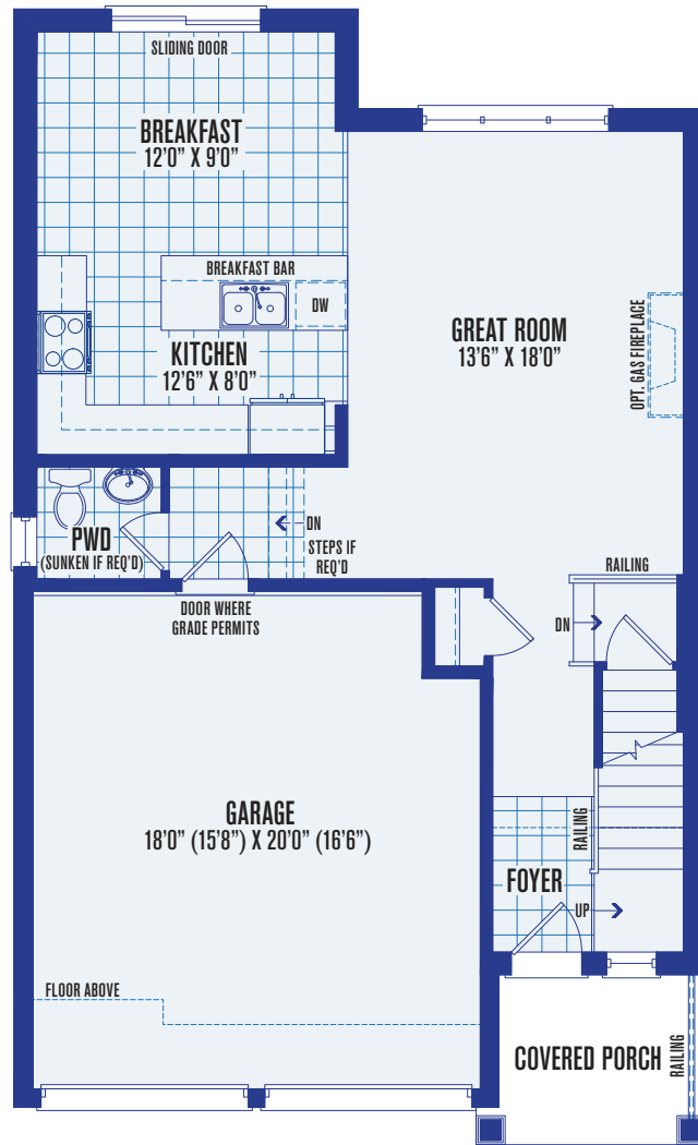
MAIN FLOOR
