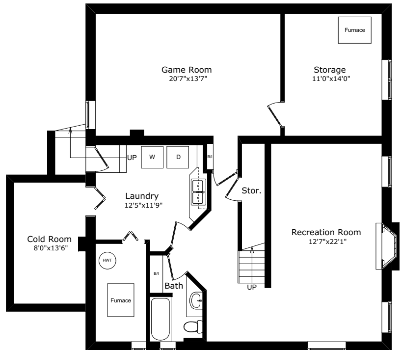
LOWER FLOOR
