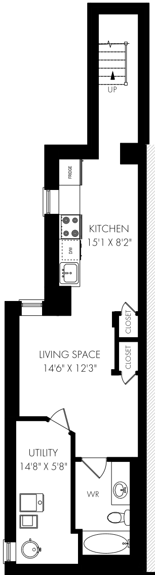
LOWER LEVEL - 666 SQUARE FEET
