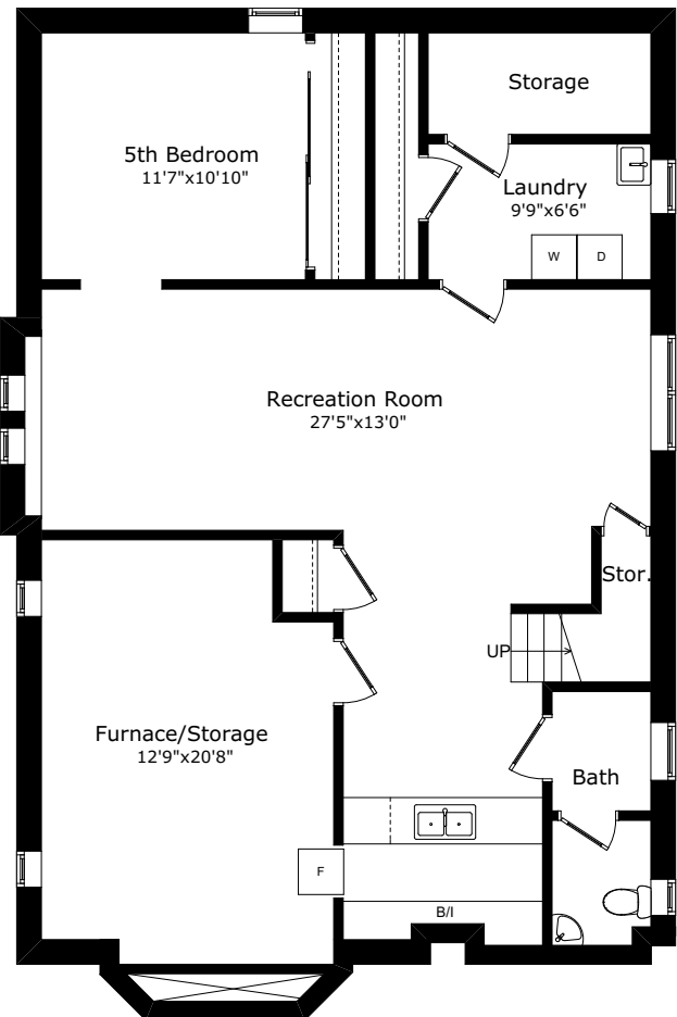
LOWER FLOOR
