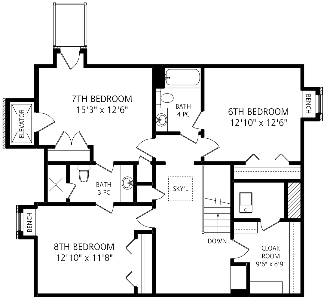
THIRD FLOOR 1,165 SQUARE FEET
