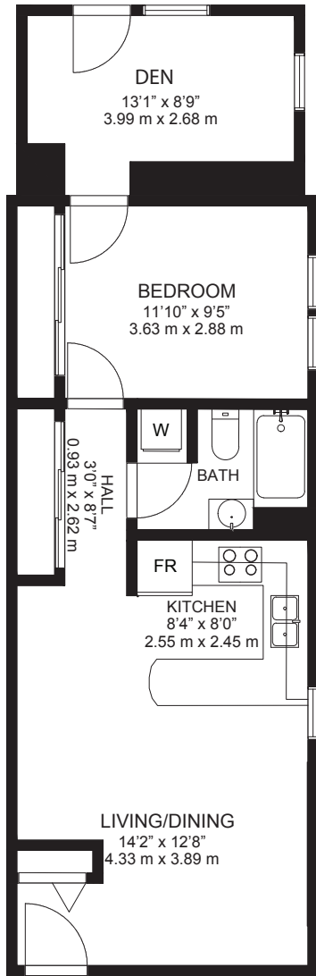
BASEMENT
